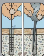
Clean drill hole
