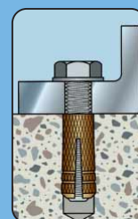
Mount component
