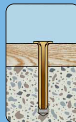
Knock in securing sleeve with mason's mallet until flush
