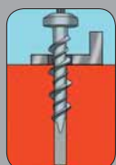
Screw in screw anchor
