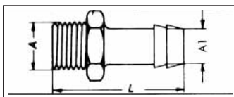
Threaded Grommet
