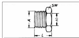
Reducing Nipples
